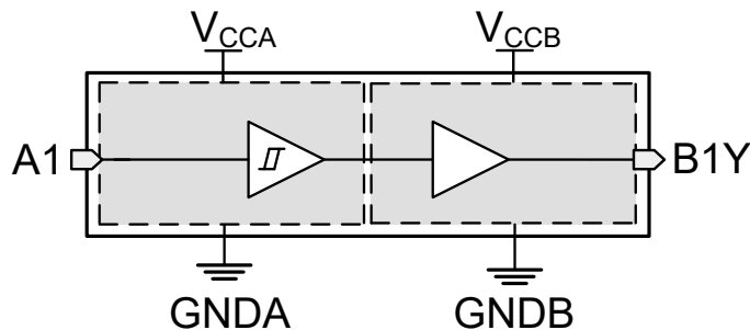
Figure 7-1. TXG8010-Q1 Functional Block Diagram
