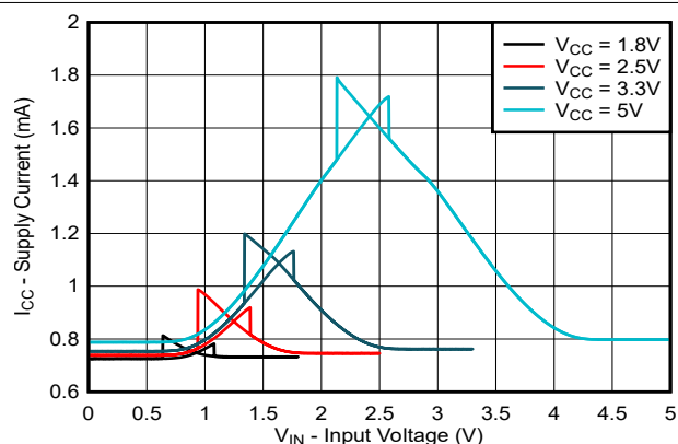
Figure 5-4. Supply Current ( I_{CC} ) vs Input Voltage ( V_{IN} ) [TXGx042]
