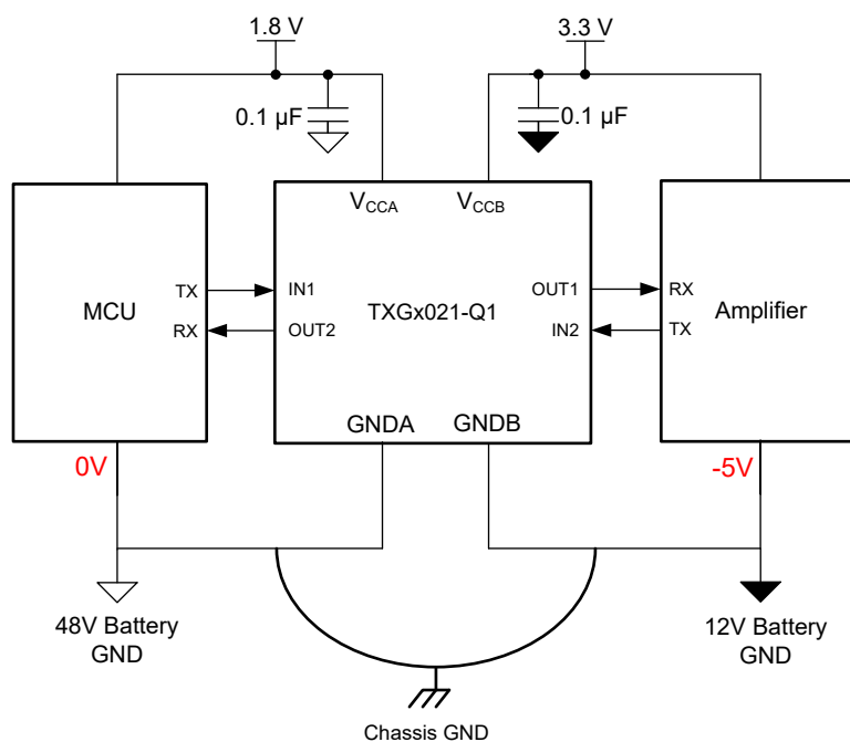
Figure 8-1. TXG1021-Q1 in Automotive
