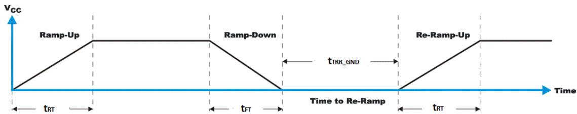
Figure 8-2. V_{CC} is lowered to 0V and then ramped up
