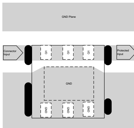
Figure 12. TVS1400 Layout
