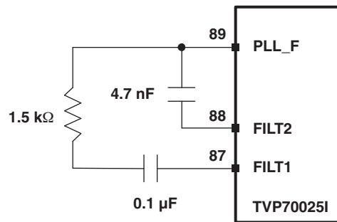
Figure 4. Horizontal PLL Loop Filter
