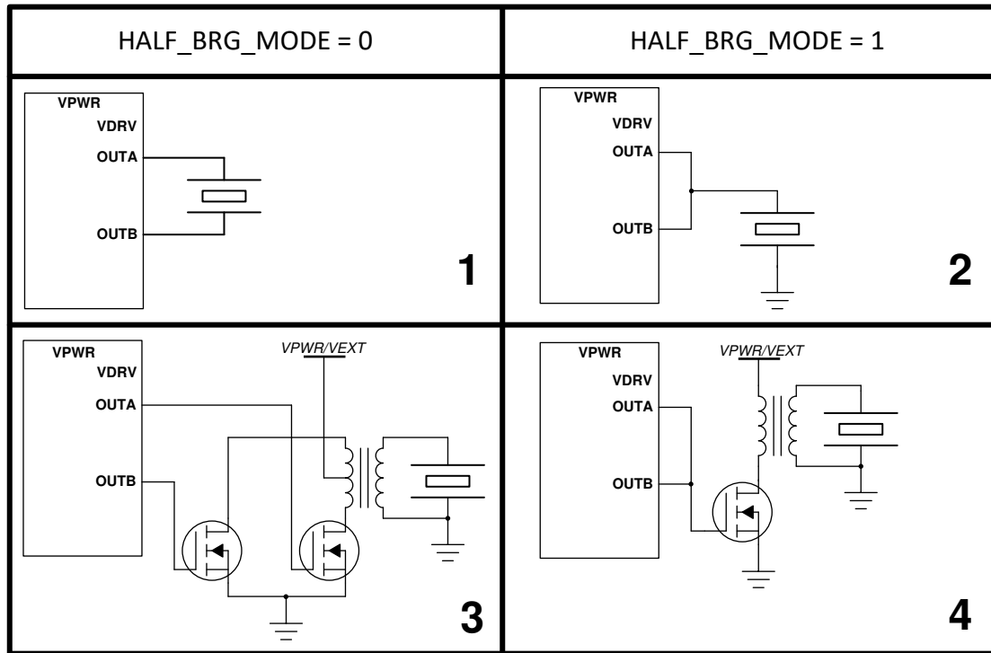
Figure 8-2. TUS4470 Transducer Drive Options
