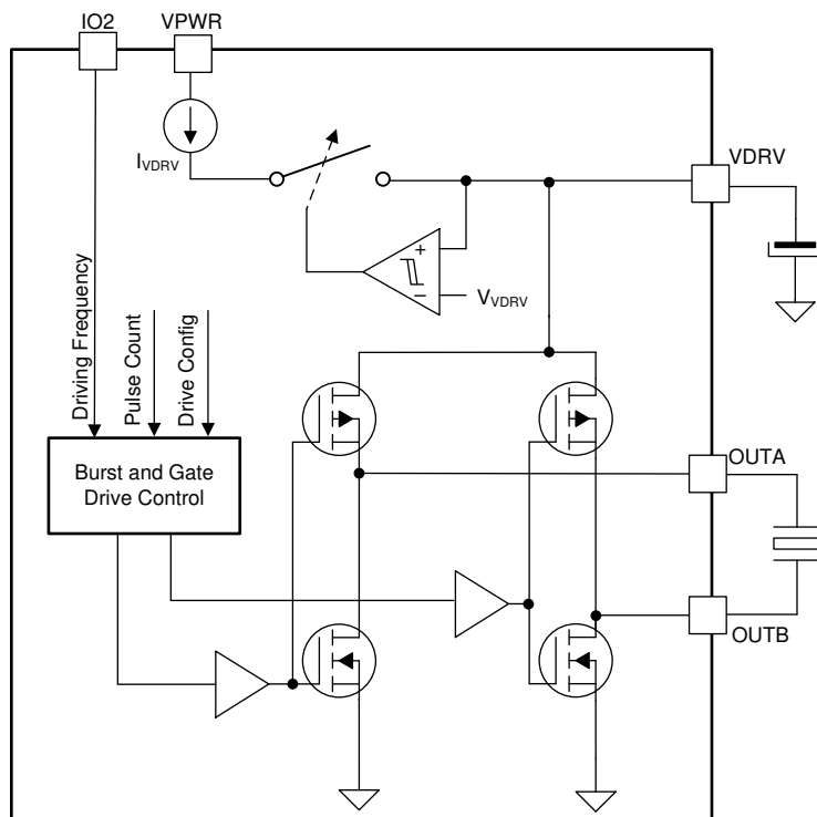
Figure 7-5. Direct Drive Configuration Using Internal FETs
