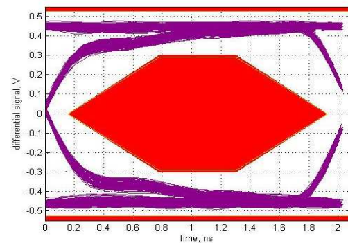
Figure 39. Downstream Port 3
