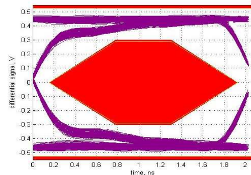
Figure 39. Downstream Port 3
