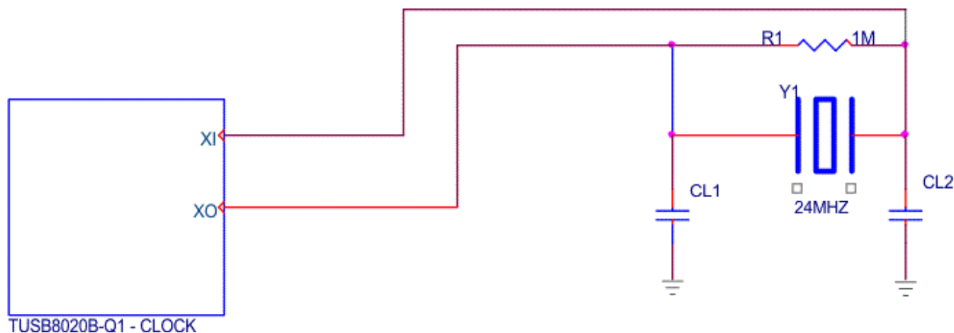
Figure 2. TUSB8020B-Q1 Clock
