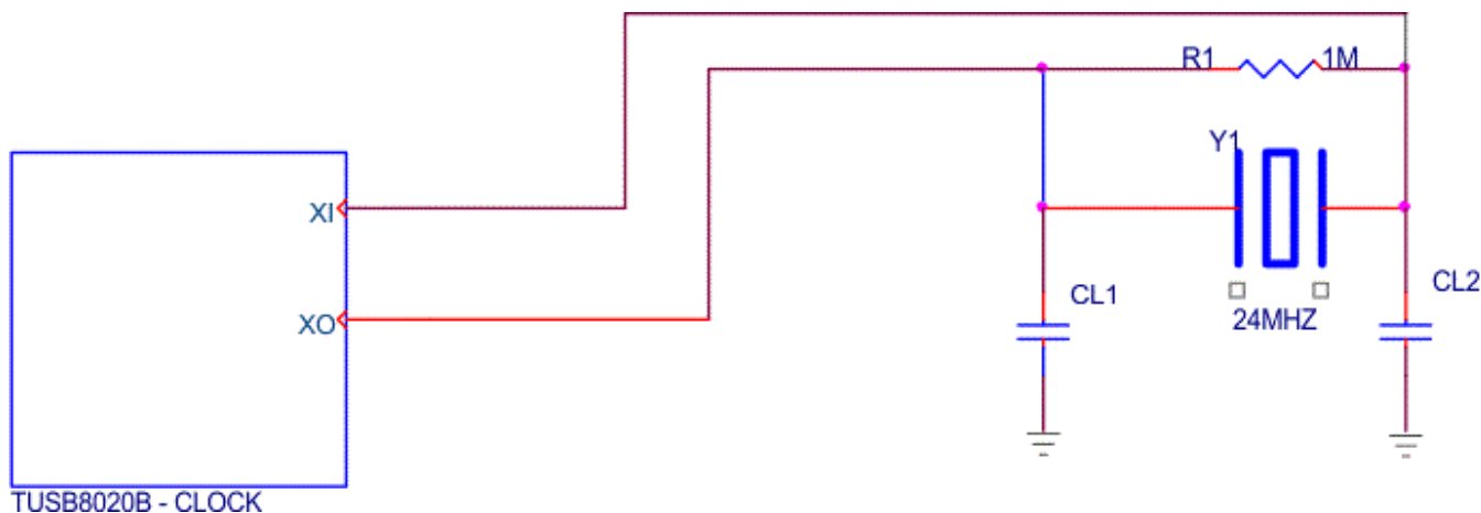
Figure 2. TUSB8020B Clock
