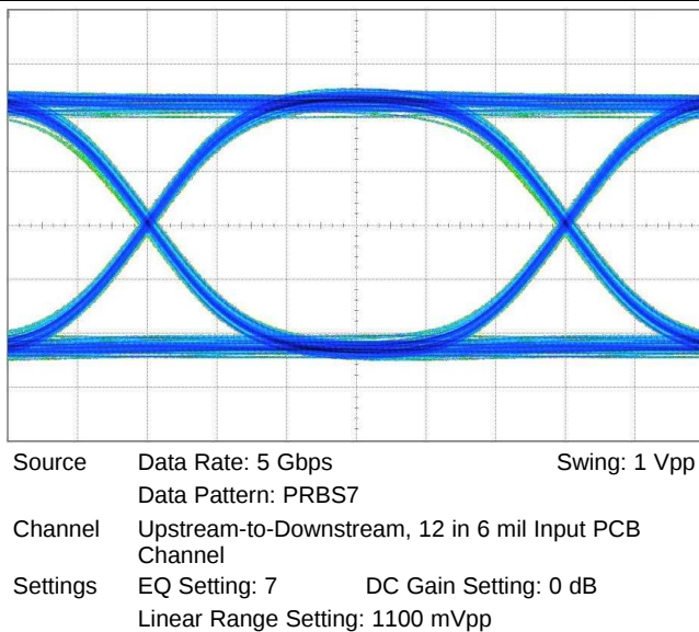
Figure 17. Output Eye-Pattern Performance at 5 Gbps
