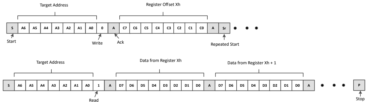
Figure 7-4. I²C Read with Repeated Start
