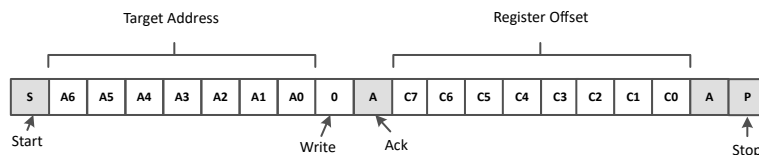
Figure 7-5. I²C Write Without Data
