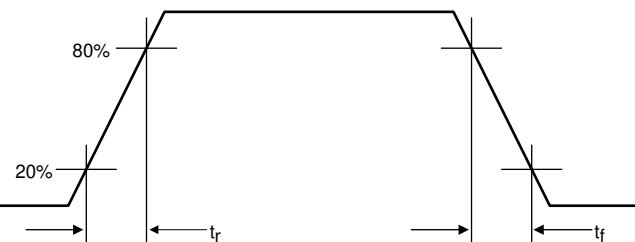
Figure 6-4. Output Rise and Fall Times
