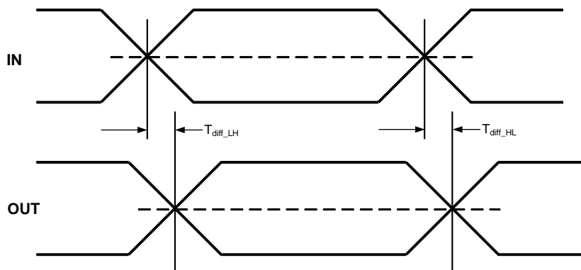
Figure 2. Propagation Delay
