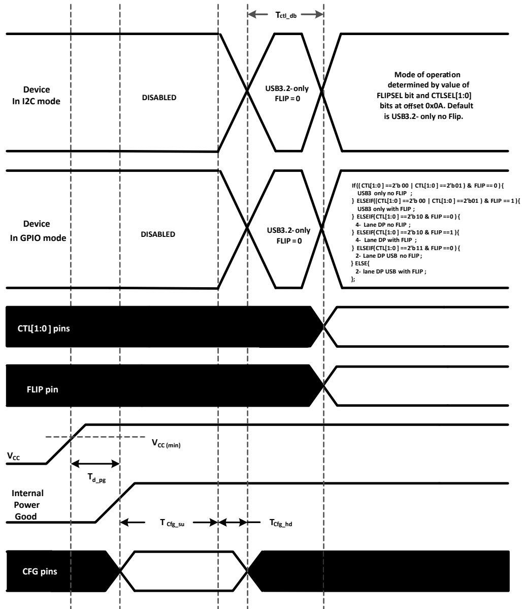
Figure 6-10. Power-On Timing
