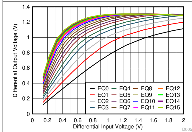
Figure 6-5. USB TX Linearity Curves at 5 GHz
