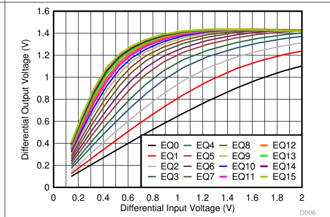
Figure 6-6. USB RX Linearity Curves at 5 GHz
