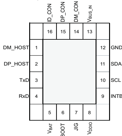
QFN-RSV PIN-OUT
