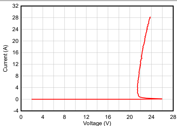
Figure 5-6. Positive TLP Curve - TSD18
