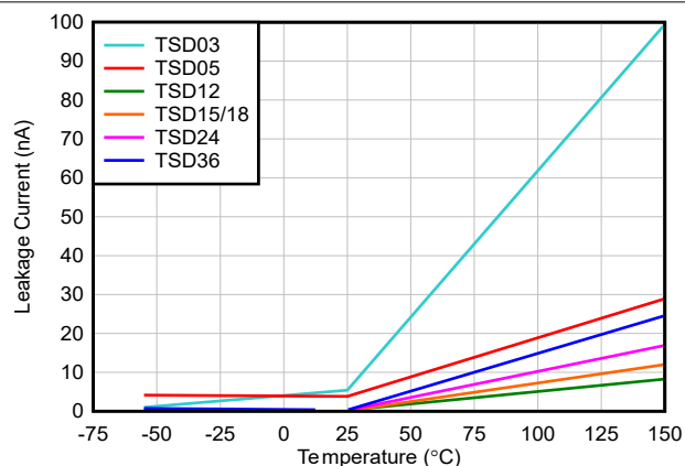
Figure 5-10. Leakage Current vs Temperature
