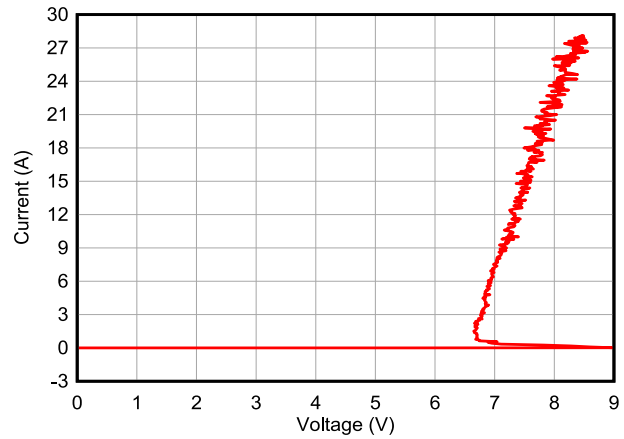
Figure 5-2. Positive TLP Curve - TSD05
