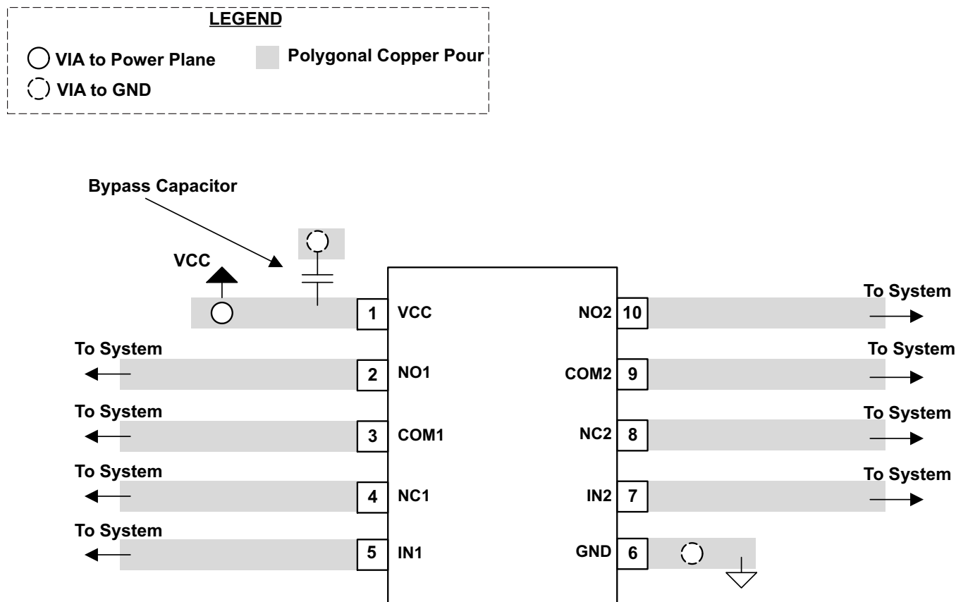
Figure 26. Layout Example of TS5A22364
