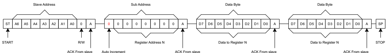
Figure 21. Repeated Data Write to a Single Register
