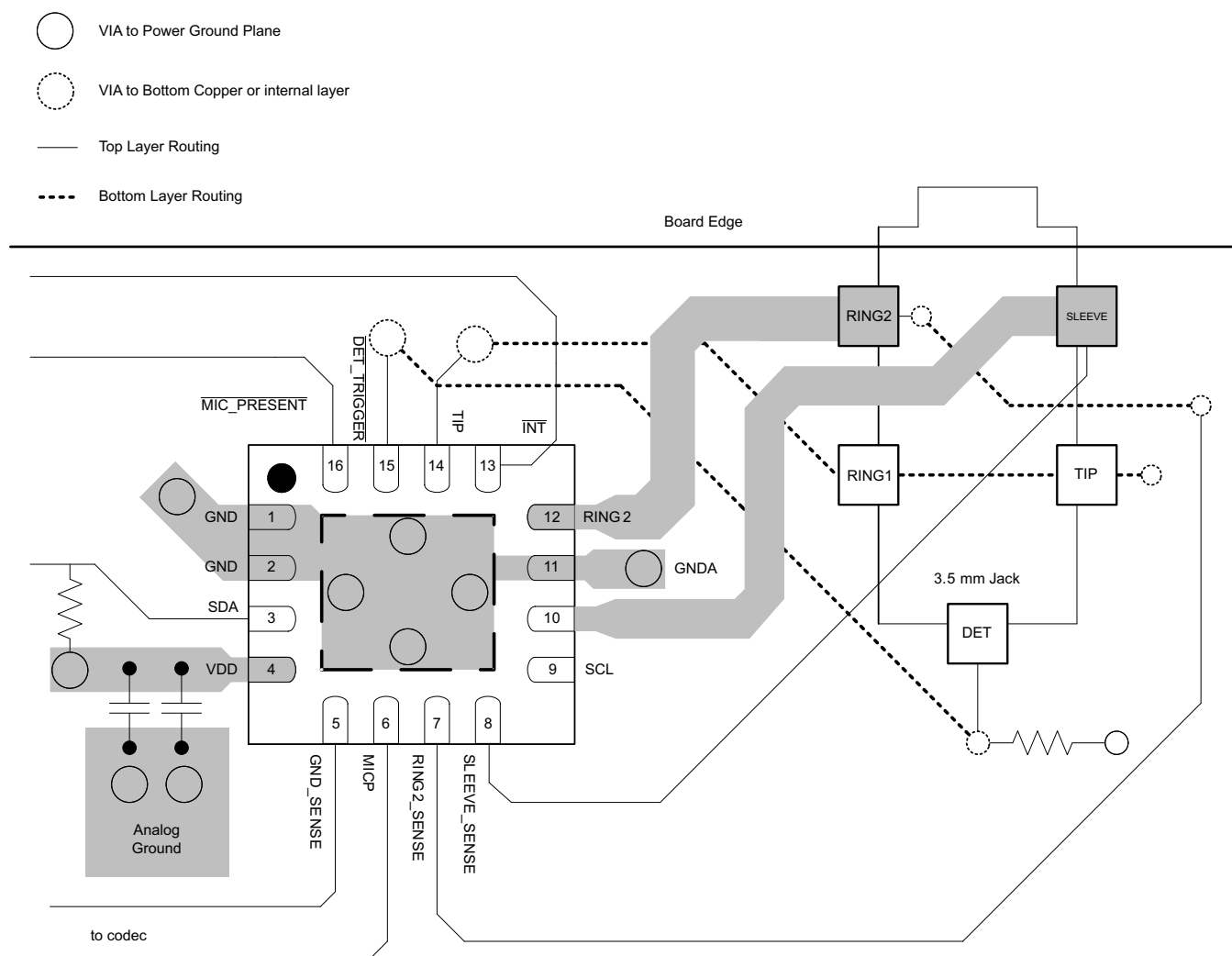
Figure 35. QFN Layout Example
