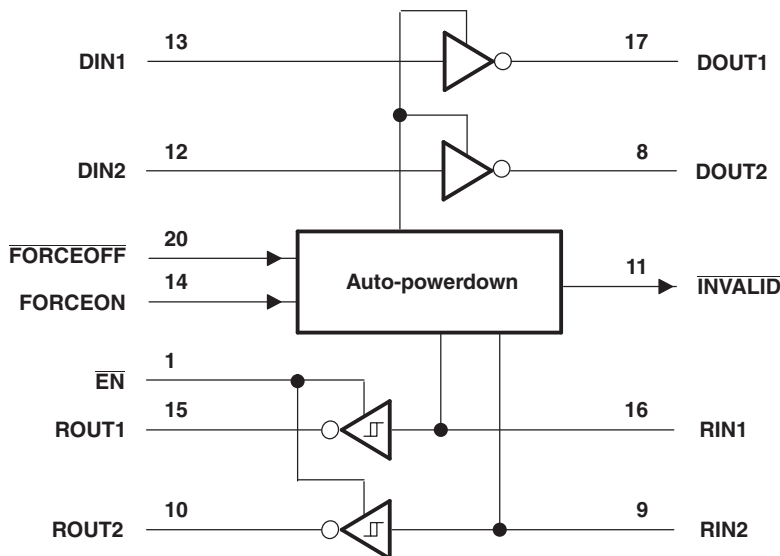
LOGIC DIAGRAM
