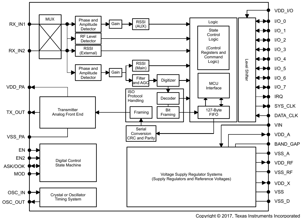
Figure 1-1. Block Diagram
