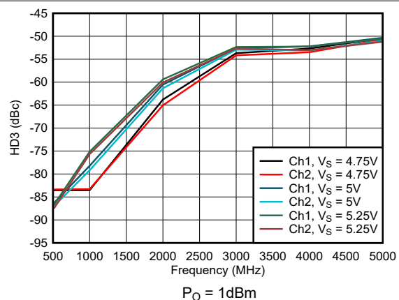
Figure 6-40. HD3 Across Supply Voltage
