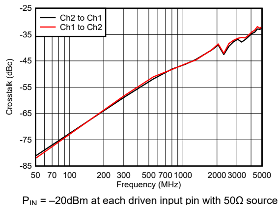
Figure 6-130. Crosstalk
