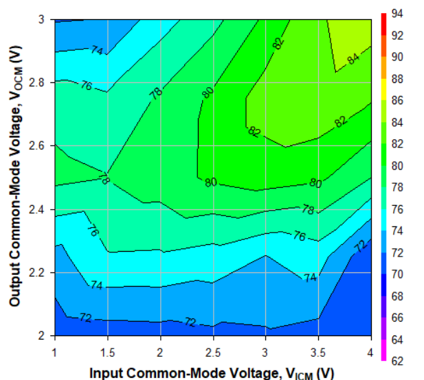
Figure 6-47. OIP3 Across V_{\text{ICM}} and V_{\text{OCM}} at 2GHz, Ch1
