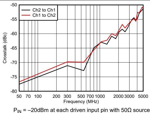
Figure 6-73. Crosstalk
