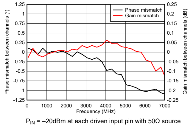
Figure 6-125. Gain and Phase Mismatch Between Channels
