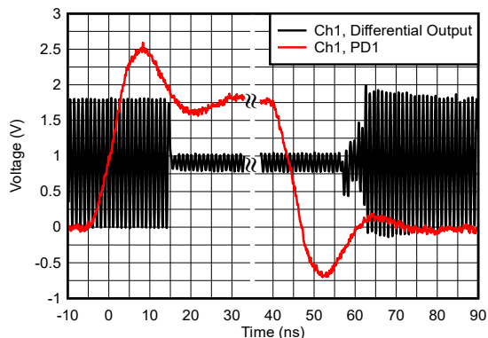
Figure 6-118. Step Response
