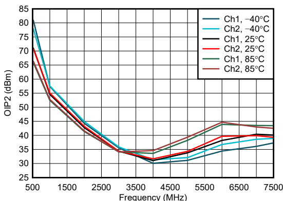
Figure 6-94. OIP2 Across Temperature
