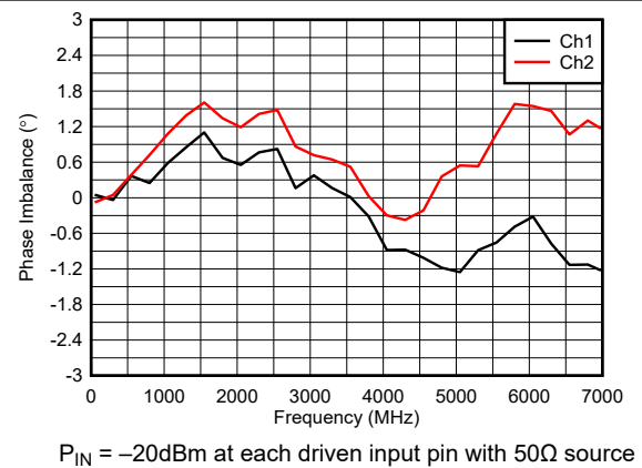
Figure 6-127. Phase Imbalance
