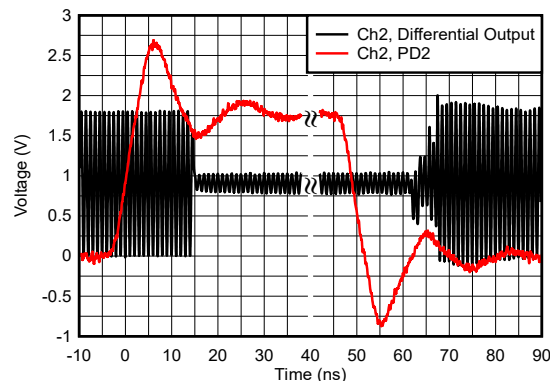
Figure 6-119. Step Response
