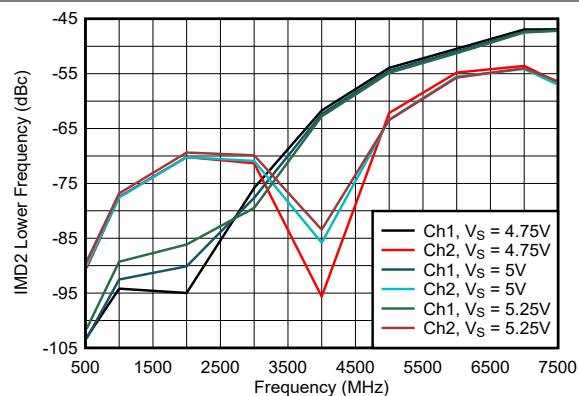
Figure 6-26. IMD2 Lower Across Supply Voltage
