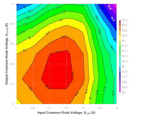
Figure 6-16. OIP3 Across V_{\text{ICM}} and V_{\text{OCM}} at 2GHz
