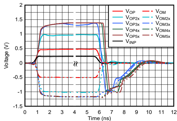
S2D, dc-coupled, V_{S+} = 2.5\text{V} , V_{S-} = -2.5\text{V} , 2x to 5x output voltages are with an input voltage 2 to 5 times that of V_{\text{INP}} as shown, respectively
