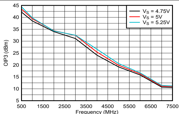
Figure 6-8. OIP3 Across Supply Voltage
