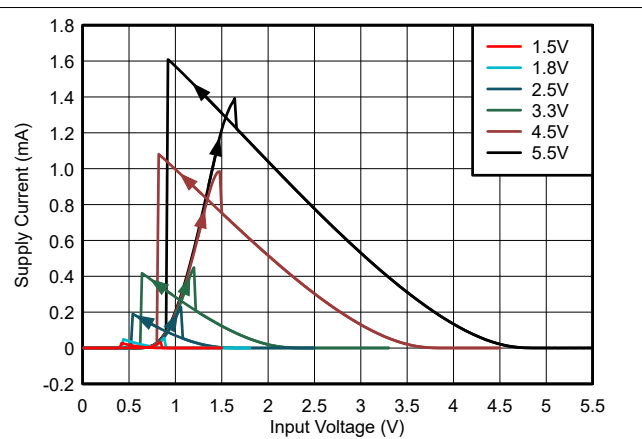
Figure 5-2. Supply Current vs Input Voltage
