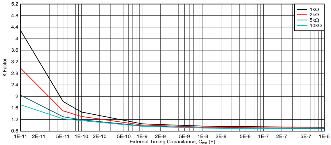
Figure 5-17. K Factor, V_{CC} = 5.5V , R_{ext} = 1k\Omega to 10k\Omega
