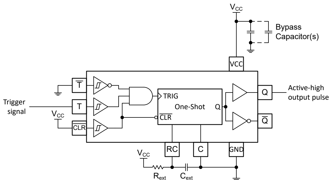
Figure 8-1. Pulse Generator Schematic Using the TPUL2T123
