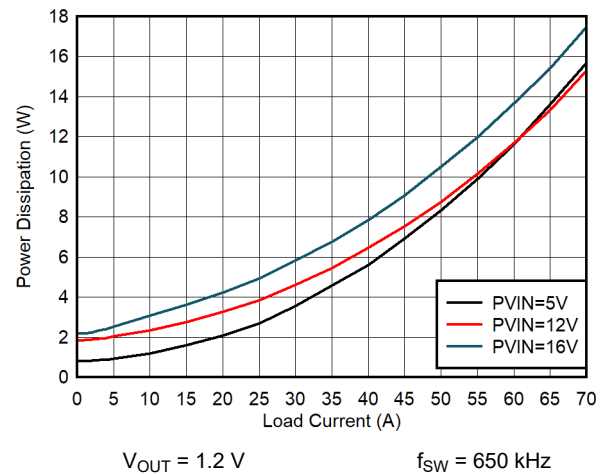
Figure 9-14. Power Dissipation
