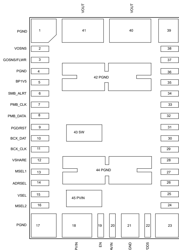
Figure 6-1. 45-Pin QFM-MOY Package (Top View)
