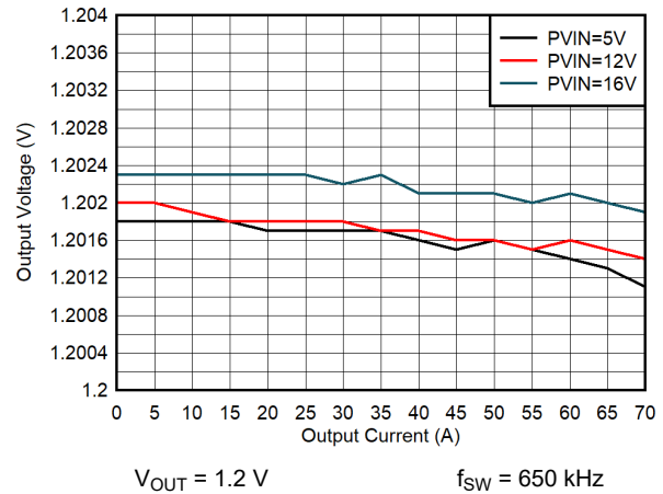
Figure 9-12. Load Regulation
