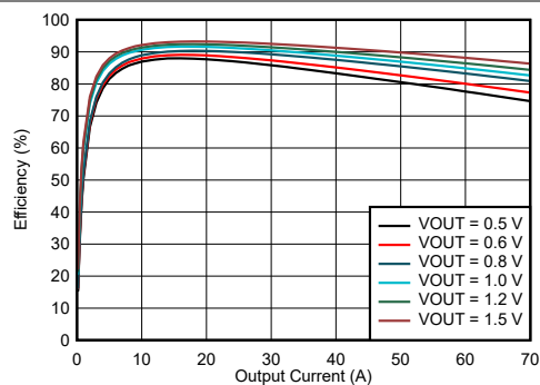
Figure 5-1. TPSM8D6C24 Efficiency vs Output Current
