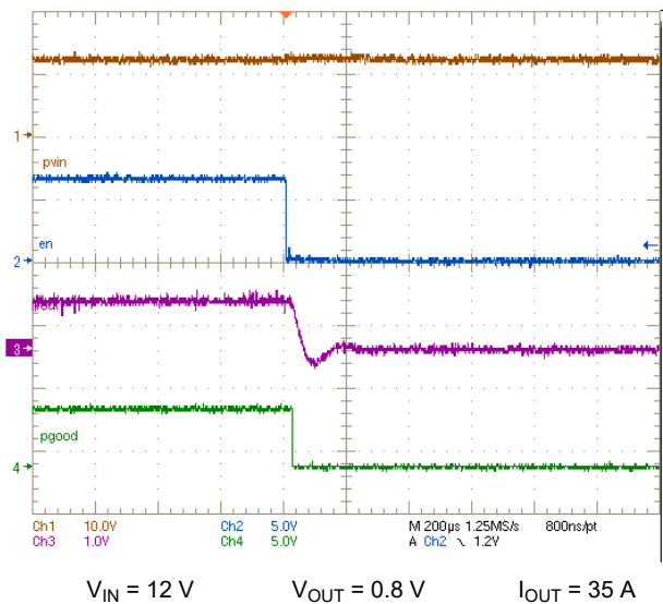
Figure 7-6. Shutdown from CNTL
