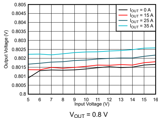
Figure 7-3. Line Regulation
