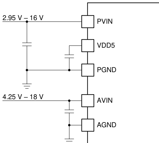
Figure 6-2. TPSM8D6C24 Separate PVIN and AVIN Connections
