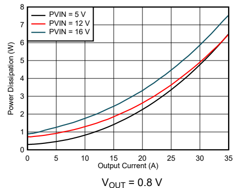
Figure 7-4. Power Dissipation
