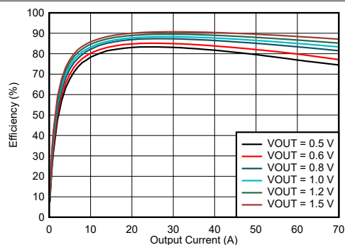
Figure 5-1. TPSM8D6C24 Efficiency vs Output Current
