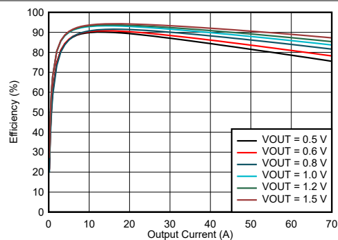
Figure 5-2. TPSM8D6C24 Efficiency vs Output Current
