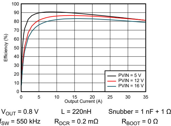
Figure 7-1. Efficiency vs Output Current
