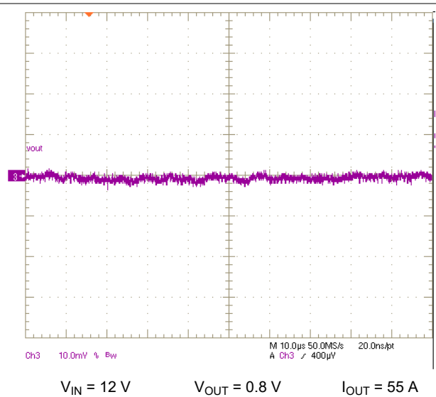
Figure 7-17. V_{OUT} Steady-State Ripple
