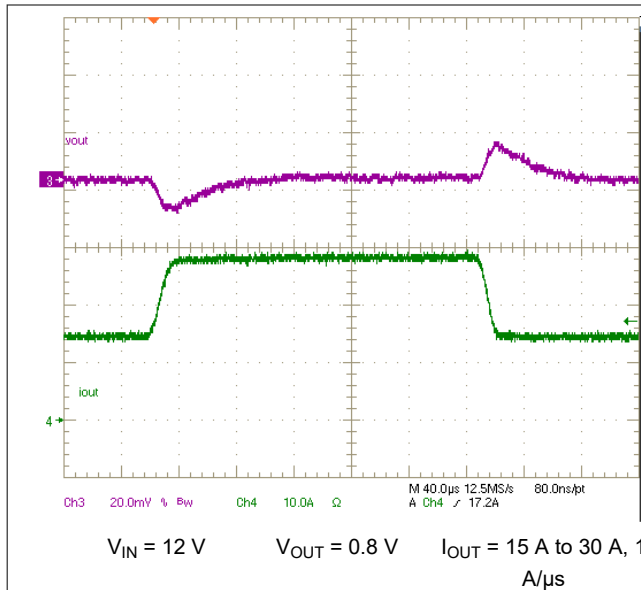
Figure 7-16. Load Transient Response
