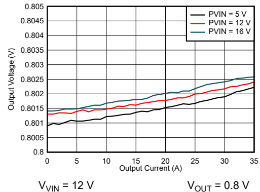
Figure 7-2. Load Regulation
