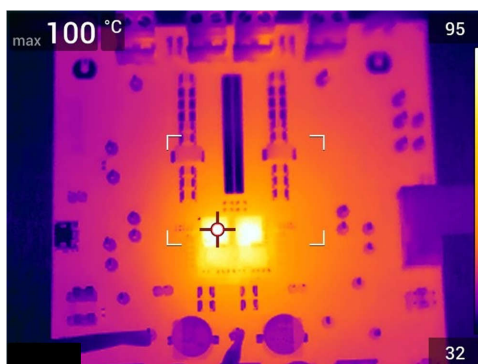
Figure 7-23. Thermal Image at 25°C Ambient, 12 Vin, 0.8V and 1.2 Vout, 35 A, 550 kHz
