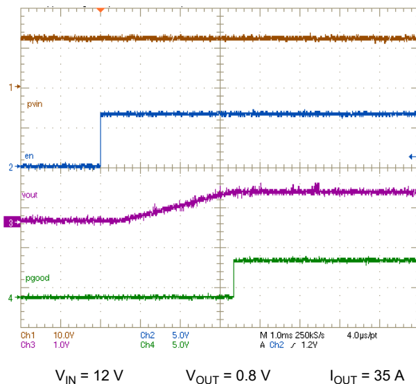
Figure 7-5. Start-Up from EN/UVLO
