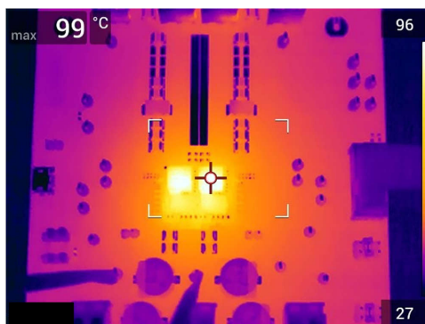
Figure 7-24. Thermal Image at 25°C Ambient, 12 Vin, 0.8 Vout, 70 A, 550 kHz
