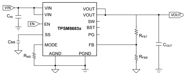
Simplified Schematic
