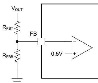
Figure 6-3. FB Resistor Divider
