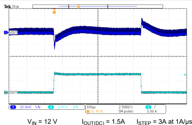
Figure 7-8. Load Transient
