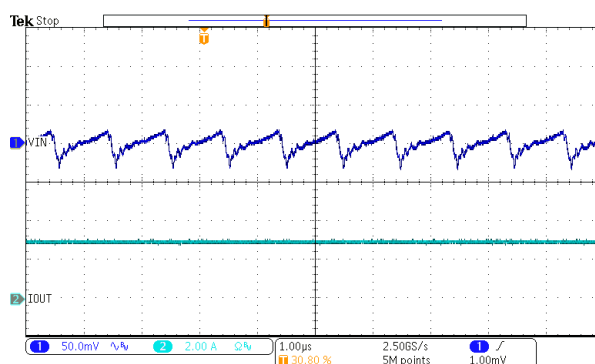
V_{IN} = 12V I_{OUT} = 3A Figure 7-18. Input Ripple – 3A Load
