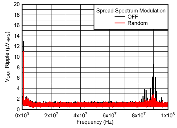
12 V to 1.8 V, 1 A 2.2 \mu\text{H} , 1 MHz First and second L-C Figure 6-8. V_{OUT} Ripple FFT After the Second L-C Filter
