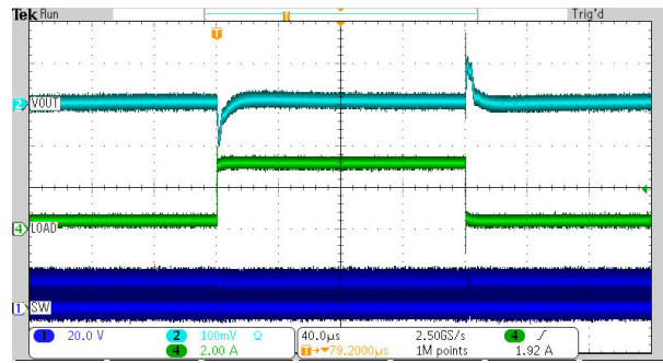
Figure 8-14. Load Transient
