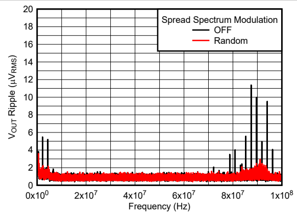
12 V to 3.3 V, 1 A 2.2 \mu\text{H} , 2.2 MHz First and second L-C Figure 6-12. V_{OUT} Ripple FFT After the Second L-C Filter
