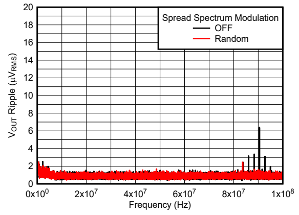
5 V to 1.8 V, 1 A 2.2 \mu\text{H} , 2.2 MHz First and second L-C Figure 6-20. V_{OUT} Ripple FFT After the Second L-C Filter
