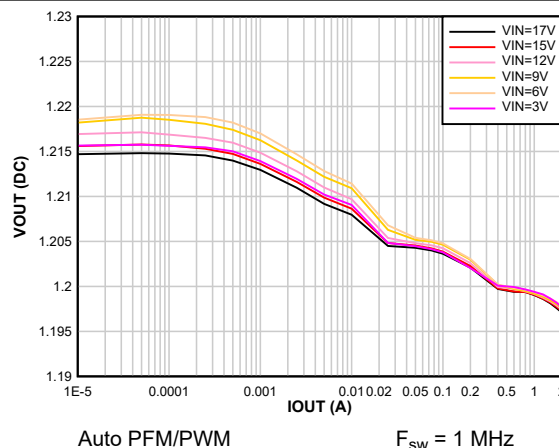
Auto PFM/PWM F_{sw} = 1 \text{ MHz} Figure 8-59. Output Voltage vs Output Current V_{OUT} = 1.2 \text{ V}
