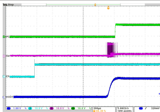
V_{IN} = 12 \text{ V} 1\text{-MHz Auto PFM/PWM} I_O = 1 \text{ A} V_{OUT} = 1.8 \text{ V} T_A = 25^\circ\text{C}
