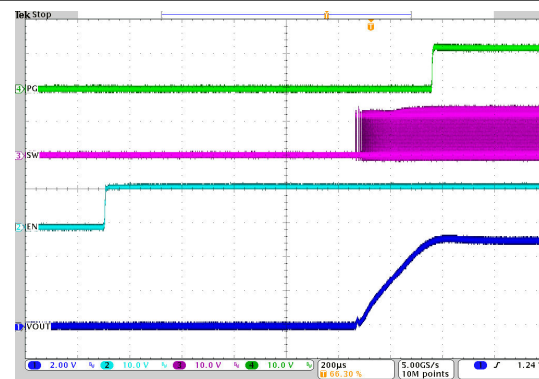
V_{IN} = 12 \text{ V} 2.5\text{-MHz FPWM} I_O = 1 \text{ A} V_{OUT} = 5 \text{ V} T_A = 25^\circ\text{C}
