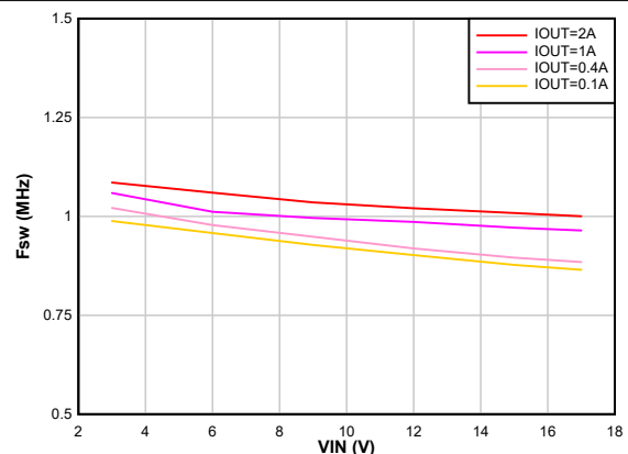
FPWM F_{sw} = 1 \text{ MHz} Figure 8-20. Switching Frequency vs Input Voltage V_{OUT} = 1.2 \text{ V}
