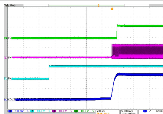
V_{IN} = 12 \text{ V} 1\text{-MHz FPWM} I_O = 0 \text{ mA} V_{OUT} = 1.2 \text{ V} T_A = 25^\circ\text{C}
