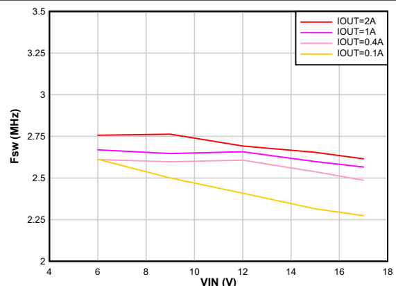
FPWM F_{sw} = 2.5 \text{ MHz} Figure 8-22. Switching Frequency vs Input Voltage V_{OUT} = 3.3 \text{ V}
