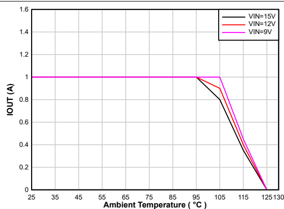
Auto PFM/PWM F_{SW} = 2.5\text{ MHz} Figure 8-46. Thermal Derating V_{OUT} = 3.3\text{ V}
