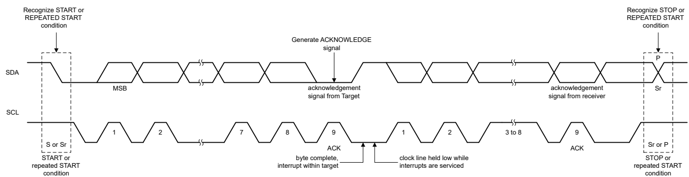
Figure 7-21. Bus Protocol
