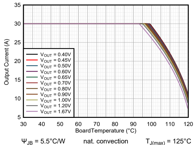
Figure 9-35. Safe Operating Area TPSM8287B30xx V_{IN} = 5.0V
