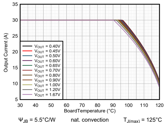
Figure 9-34. Safe Operating Area TPSM8287B30xx V_{IN} = 3.3V
