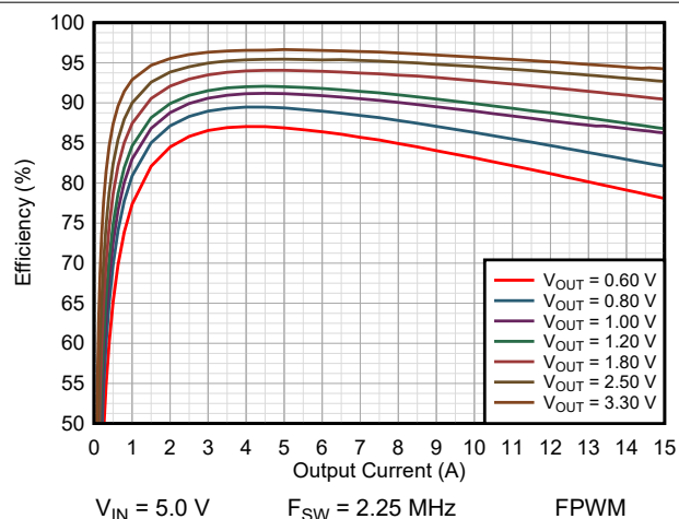
Figure 9-19. Efficiency TPSM8287A15BBH
