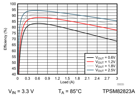
Figure 9-142. Efficiency
