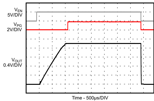
I_{OUT} = 3\text{ A} TPSM82823A
