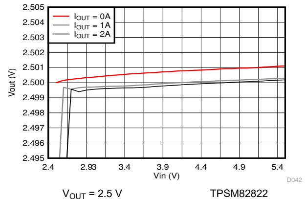
Figure 9-74. Line Regulation
