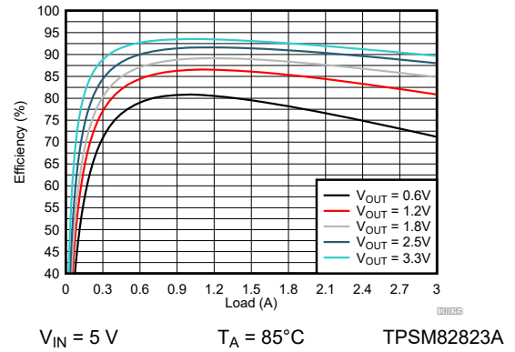
Figure 9-138. Efficiency
