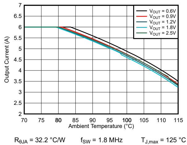
Figure 8-23. TPSM82816SIE Safe Operating Area V_{\text{IN}} = 3.3 \text{ V}
