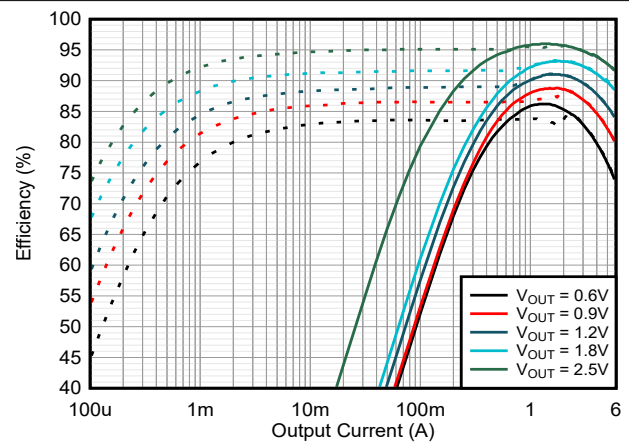
Figure 8-3. Efficiency V_{IN} = 5.0\text{ V} and T_A = 25^\circ\text{C}
