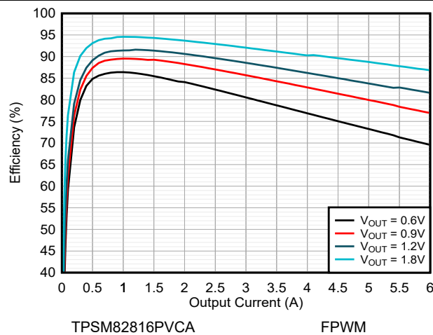
Figure 8-12. Efficiency V_{IN} = 2.7\text{ V} and T_A = 85^\circ\text{C}
