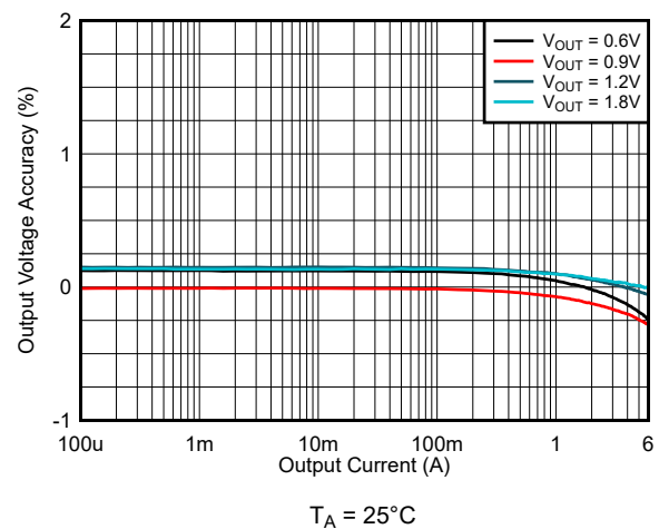
Figure 8-19. Load Regulation V_{IN} = 2.7\text{ V} (FPWM)
