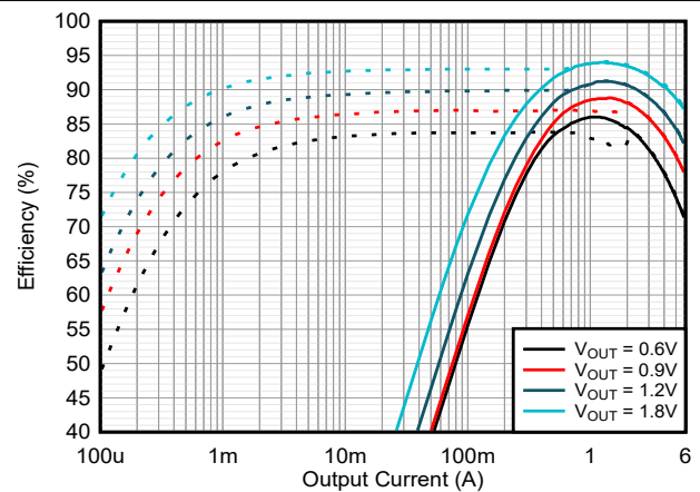
Figure 8-5. Efficiency V_{IN} = 3.3\text{ V} and T_A = 25^\circ\text{C}
