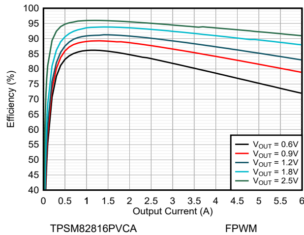
Figure 8-10. Efficiency V_{IN} = 3.3\text{ V} and T_A = 85^\circ\text{C}
