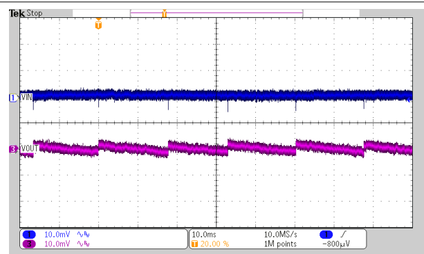
Figure 9-28. Load Transient Response
