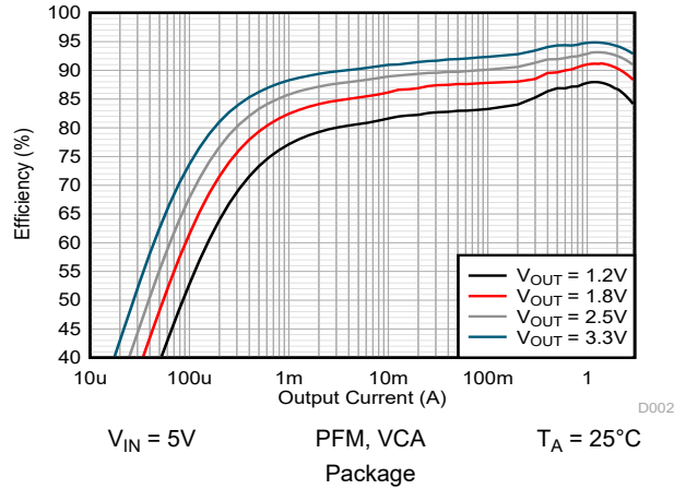
Figure 9-14. Efficiency vs Output Current
