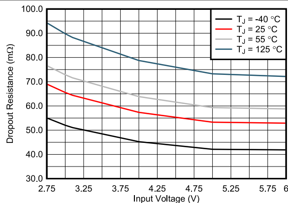
Figure 6-4. Dropout Resistance
