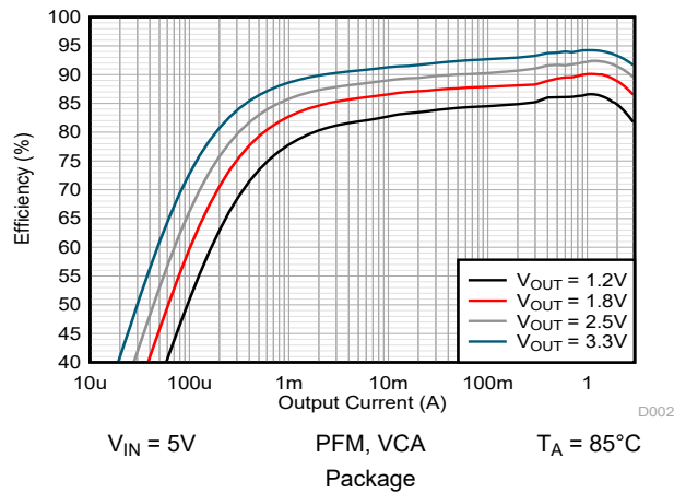
Figure 9-16. Efficiency vs Output Current
