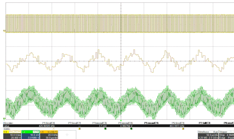
Figure 8-3. Output Ripple Without Ripple Cancellation Showing V_{\text{sw}} (Top), F_{\text{sw}} (Middle), V_{\text{out}} (Bottom)
