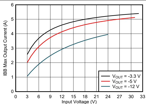
Figure 9-13. IBB Maximum Output Current
