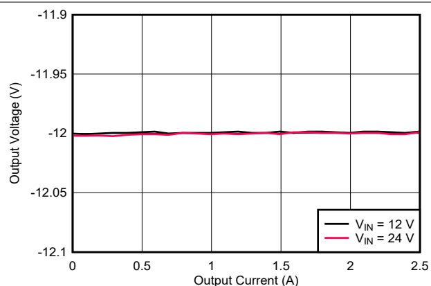
Figure 9-15. Load Regulation
