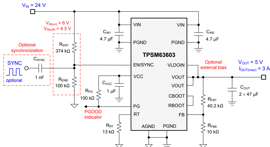
Figure 8-1. Circuit Schematic
