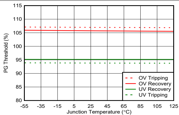
Figure 7-6. Power-Good (PG) Thresholds
