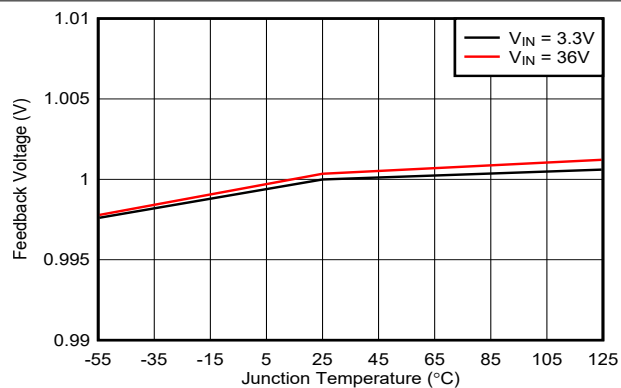
Figure 7-2. Feedback Voltage
