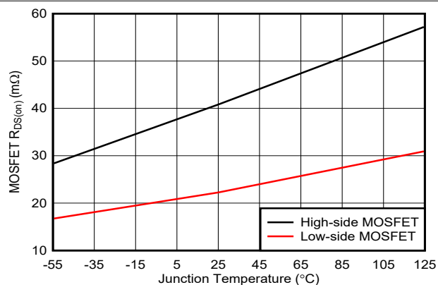
Figure 7-4. High-Side and Low-Side MOSFET R_{DS(on)}
