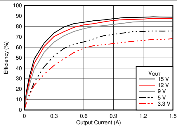
Figure 7-19. Efficiency
