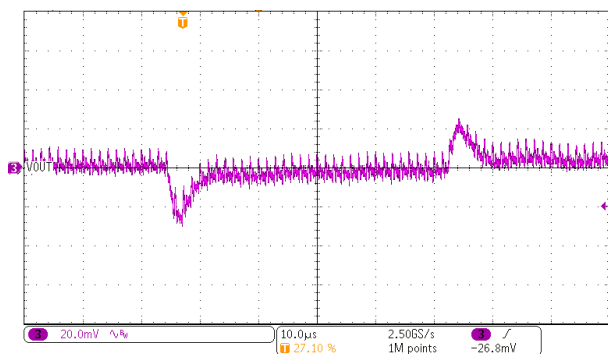
Figure 8-5. 10-A Transient Load Step
