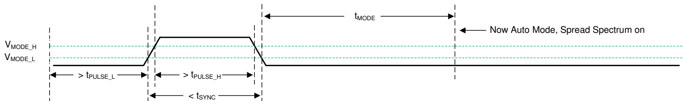
Figure 9-7. Transition from SYNC Mode to Auto Mode
