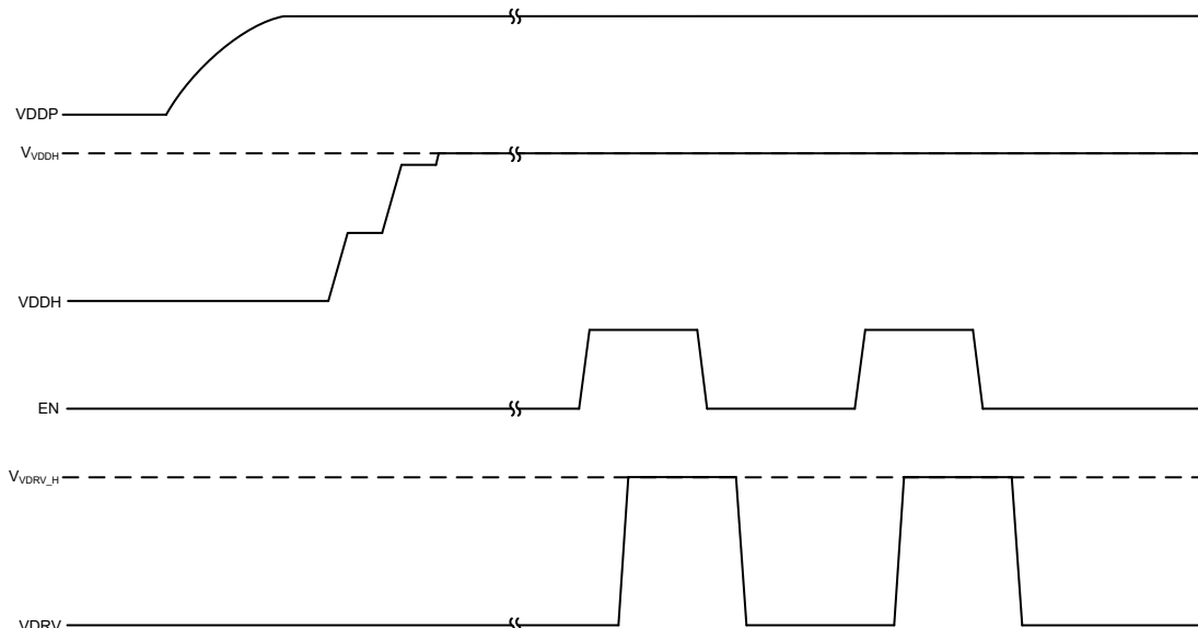
Figure 8-2. Three-Wire Mode with TPSI3052 (Standard Enable)
