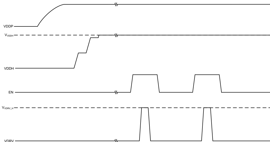
Figure 8-3. Three-Wire Mode with TPSI3052S (One-shot Enable)
