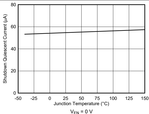
Figure 7-1. Shutdown Supply Current vs. Temperature
