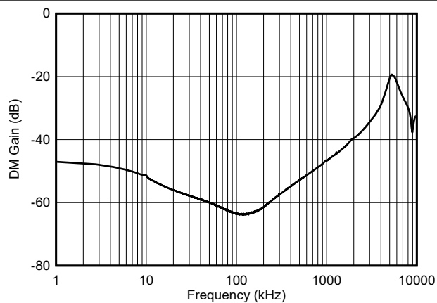
Figure 7-6. Input Filter Response – Differential Mode
