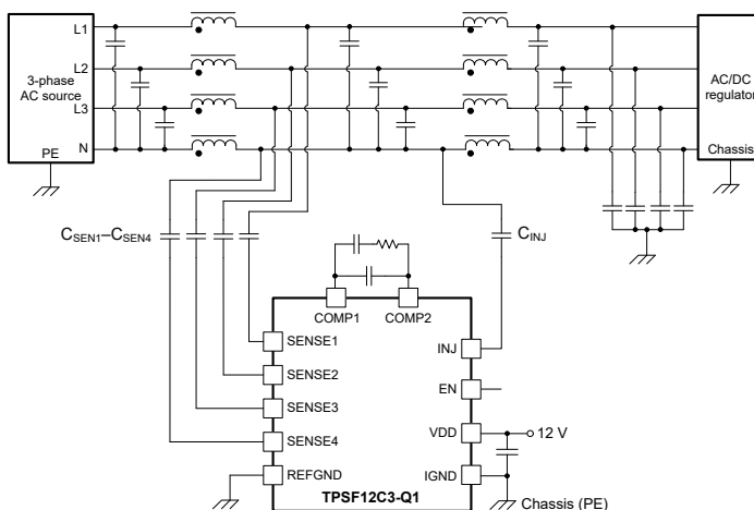
Simplified Schematic
