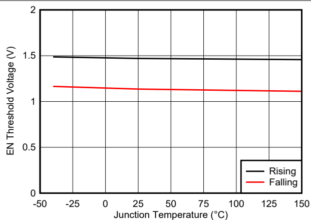
Figure 7-4. EN Threshold vs. Temperature
