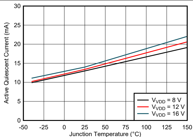
Figure 7-2. Quiescent Supply Current vs. Temperature
