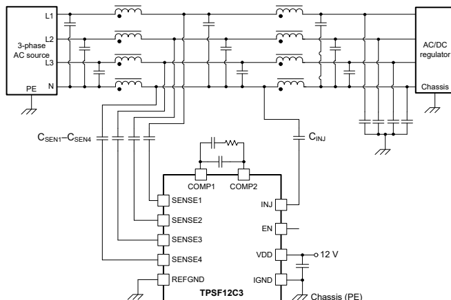
Simplified Schematic
